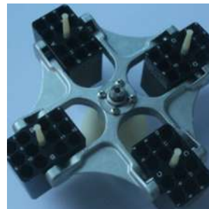
HORIZONTAL ROTOR 48 X 5ML
